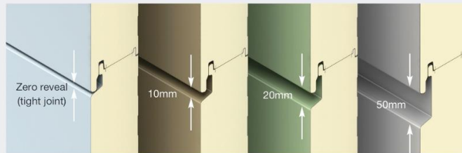
Side Joint Reveal Details Horizontal Application
